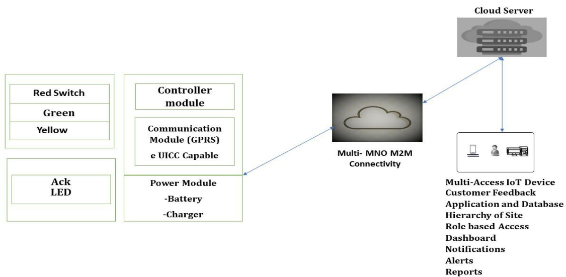
Fig.1 Feedback device architecture
